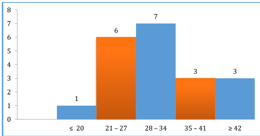
Figure 2. Shooting Histogram
